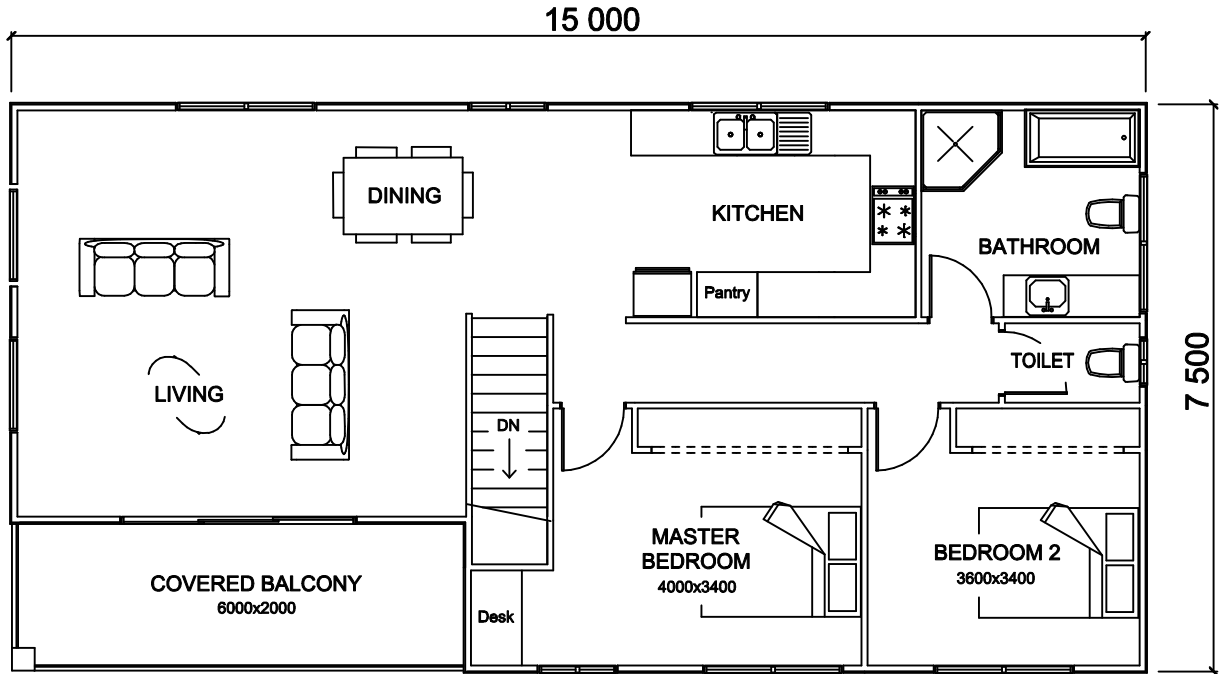
SECOND FLOOR
