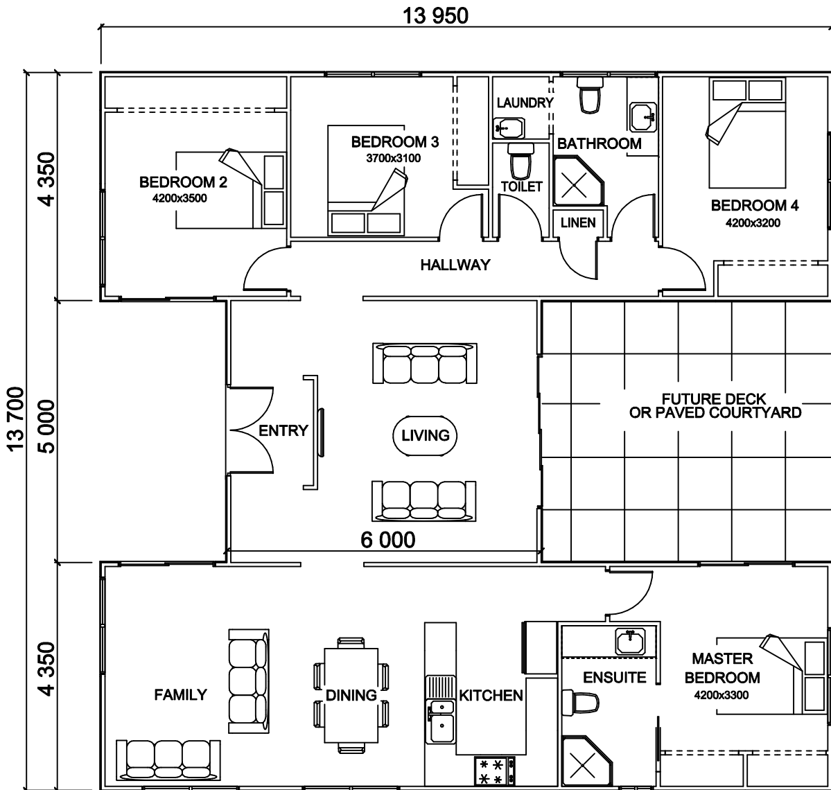
FLOOR PLAN
