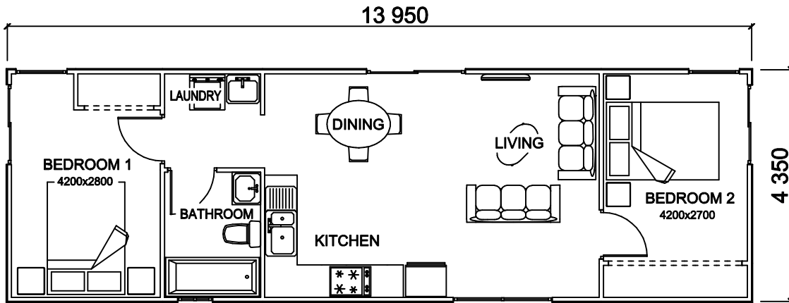
FLOOR PLAN
