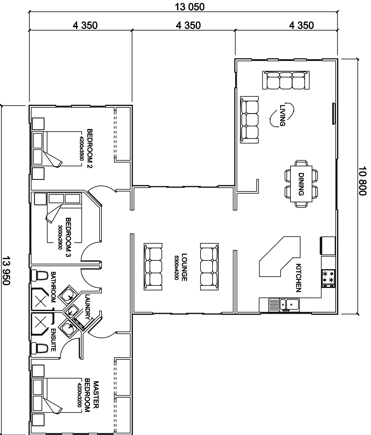
FLOOR PLAN
